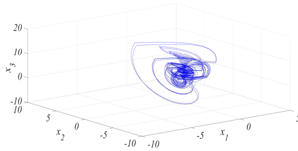
Figure 1: The hyperchaotic attractor of the system (4.1)
