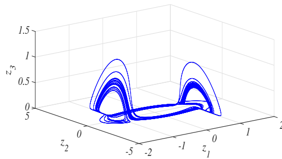
Figure 3: The chaotic attractor of the system (4.7)
