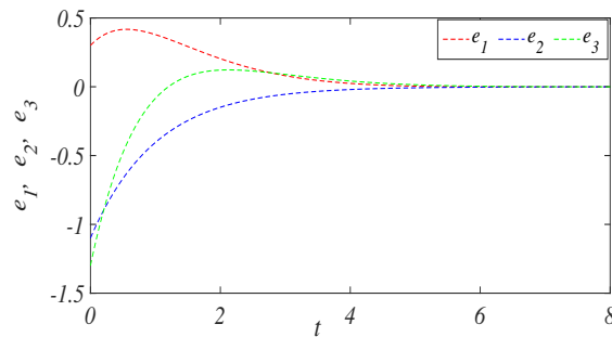
Figure 4: Time evolution of the RGCS error (4.9).
