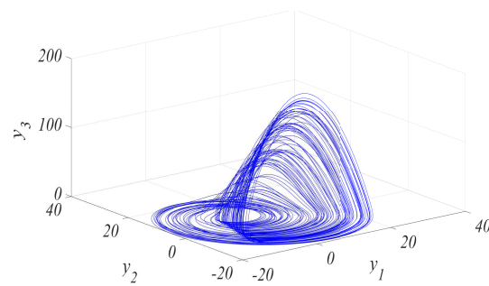
Figure 2: The hyperchaotic attractor of the system (4.4)
